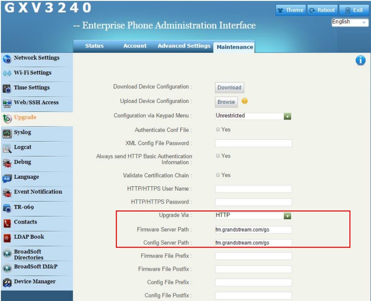
Figure 17: Upload GXV3240 Firmware via Web GUI
