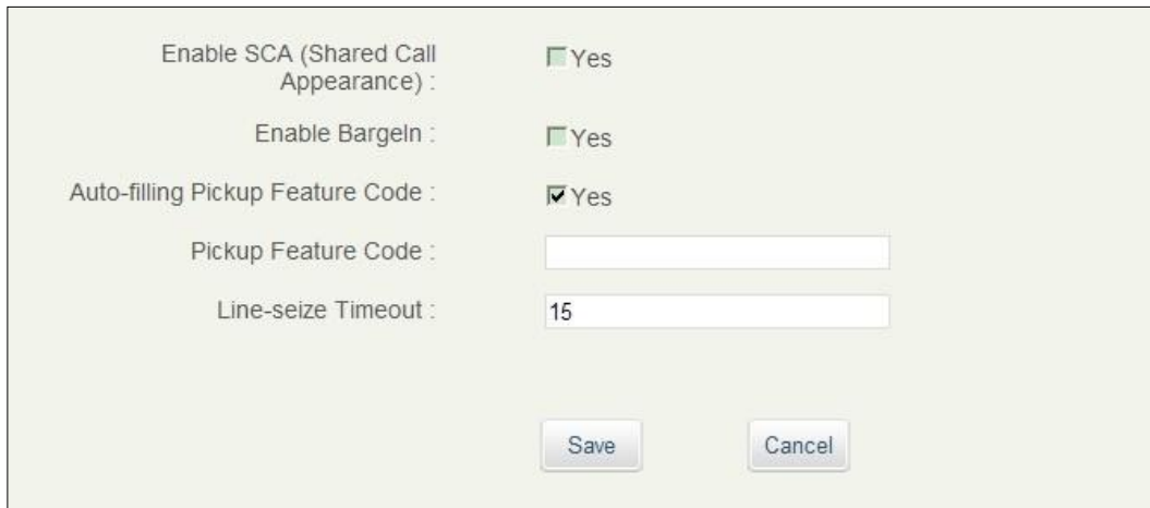
Figure 69: GXV3275 SCA Settings on Web UI
