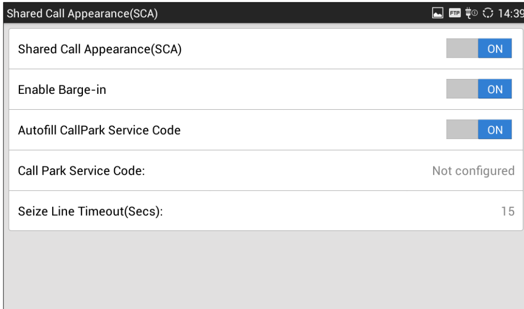
Figure 68: GXV3275 SCA Settings on LCD
