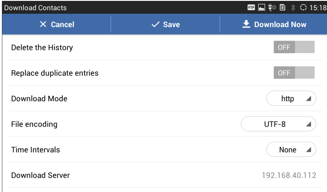
Figure 75: GXV3275 Contacts - Download Contacts
