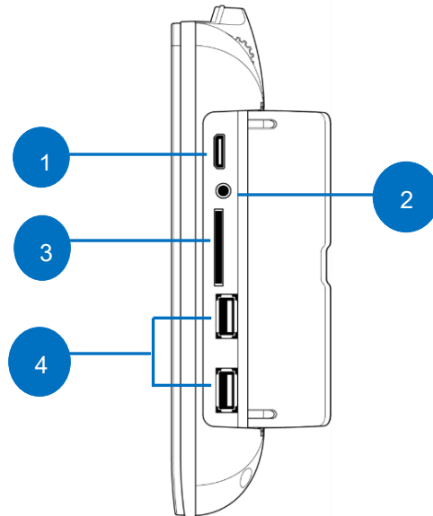
Figure 3: GXV3275 Side View
